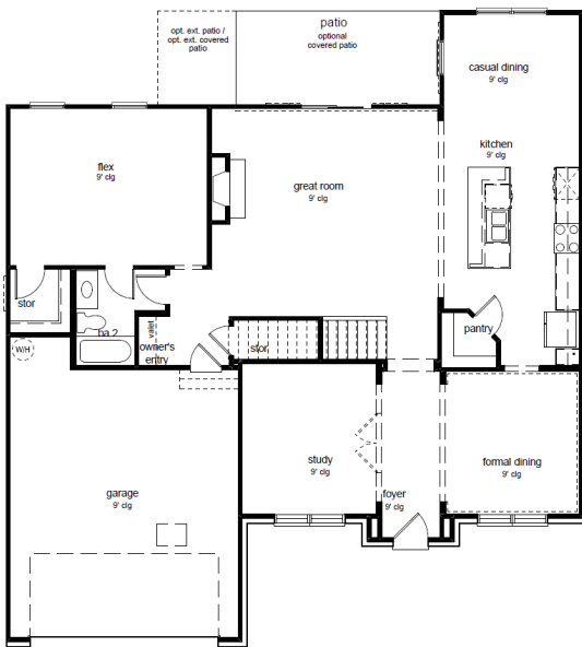
first floor plan with opt. flex i.l.o. bedroom 5
