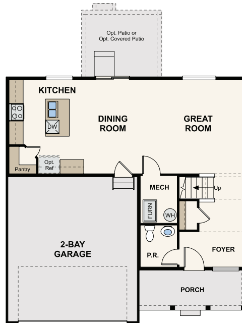
MAIN LEVEL
