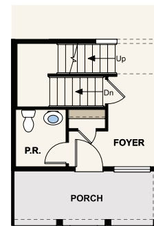
STAIRS TO OPT. FULL LOWER LEVEL
